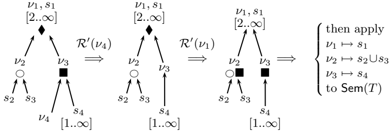
Fig. 5. Use of \mathcal{R}' on an itree and quantifier elimination
