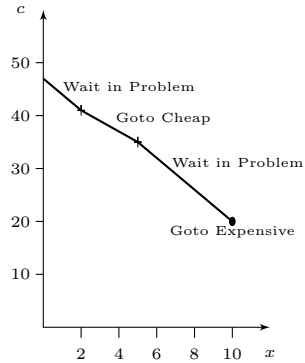
Fig. 2. Minimum cost of repair and associated strategy in location Problem
